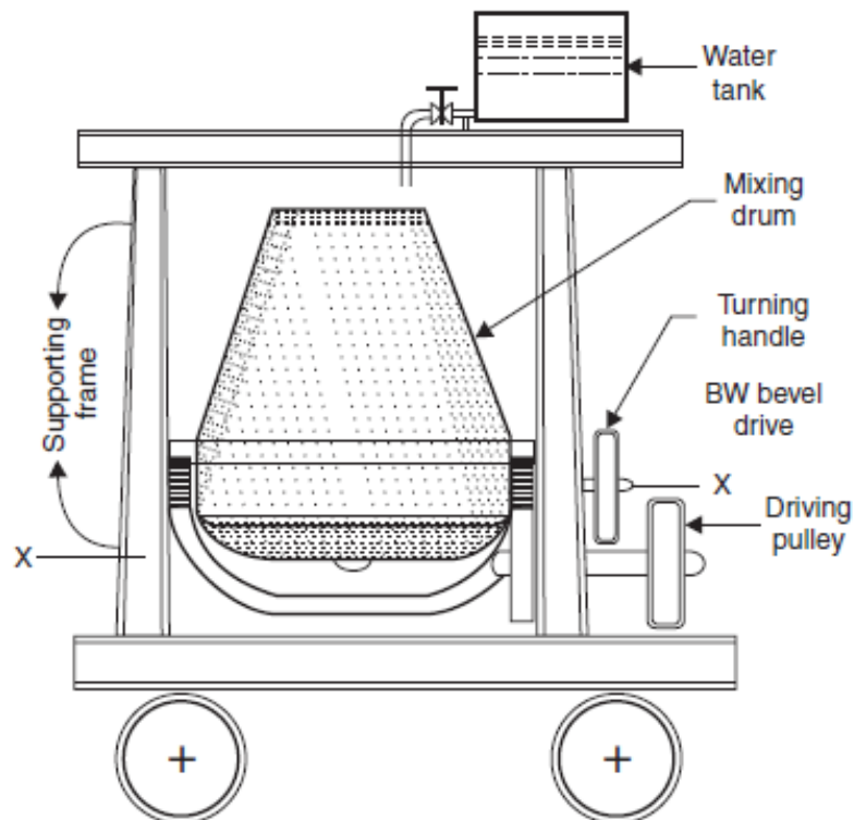
Figure 1. Concrete mixer
